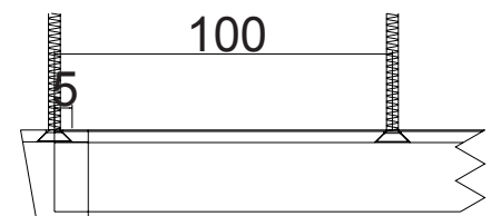
4. Distance between screw holes and end stops shall not exceed 100 mm.
