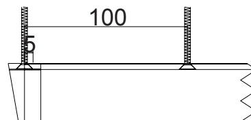
3. Distance between screw holes and end stops shall not exceed 100 mm.
